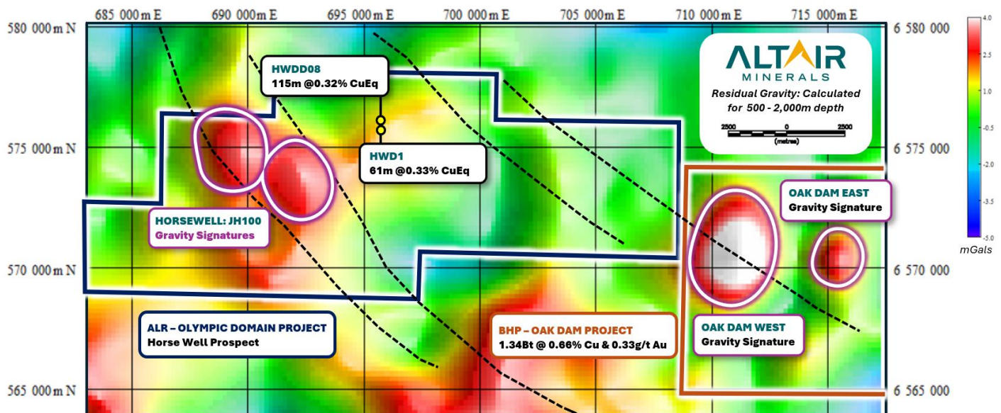
Figure 1: Residual Gravity Survey, calculated to 500-2,000m depth (BgRes), BHP Retention License shown in orange, ALR Exploration Licenses shown in blue. Major parallel northwest to southeast fault structures shown in black dotted lines. See references for further details 4,8 .
