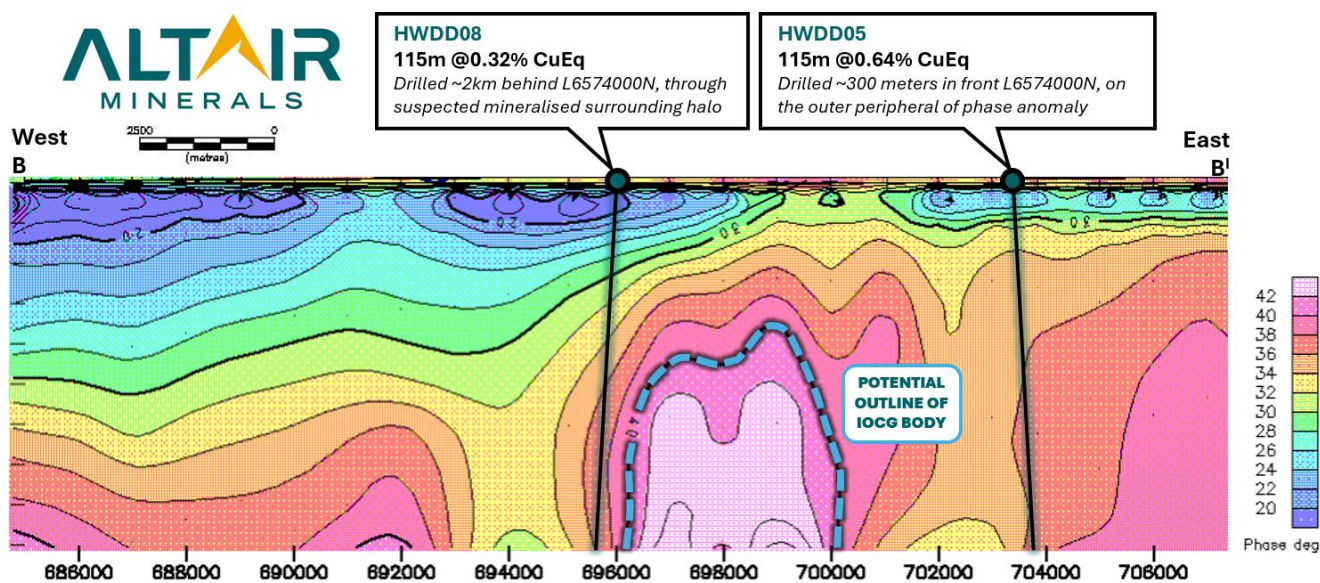
Figure 4: 3D Forward AMT Model for Phase Anomaly, cross section L6574000N (looking north). Historic holes shown 4,6 , HWDD08 superimposed onto cross section to show spatial distance from phase anomaly. Vertical scale arbitrarily modelled. Model generated by Adelaide Mining Geophysics Pty Ltd (Jim Hanneson).
